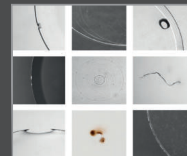
Defect visualization: bright field, dark field, telecentric illumination
